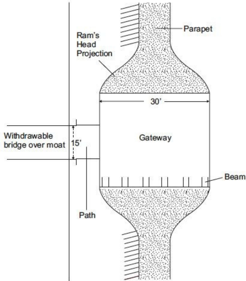
Fig. 13 Gateway-Cross-section
